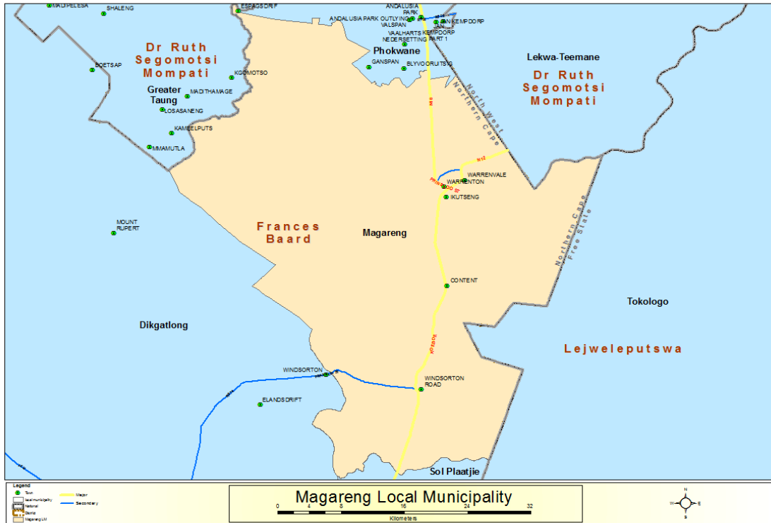
Figure 1: Location map of Magareng Local Municipality.
